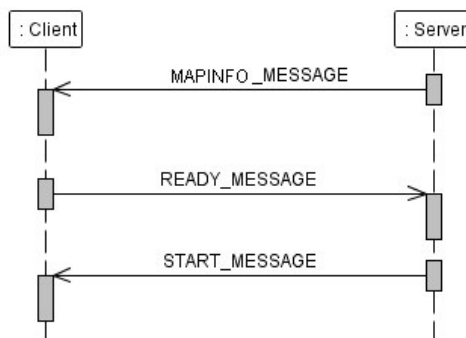
Figure 5- Starting game in two-player mode scenario
